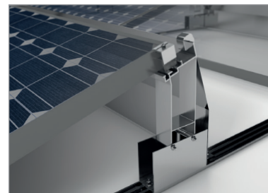
Detail back support
