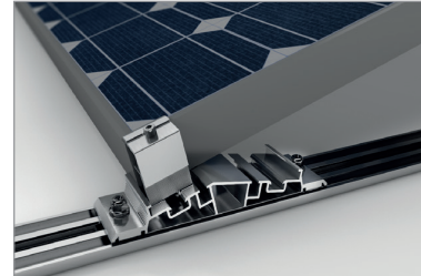
Detail front support
