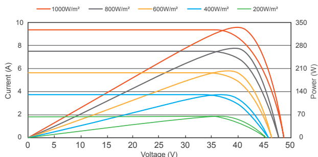
I-V&P-V curve(DH-DG-M72T/72W)
